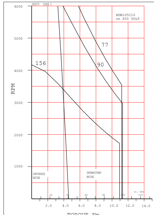
Performance Curve 650V
