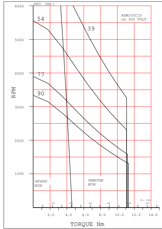
Performance Curve 300V
