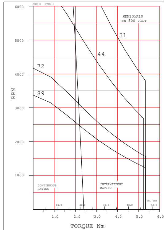
Performance Curve 300V
