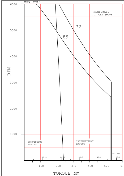
Performance Curve 560V
