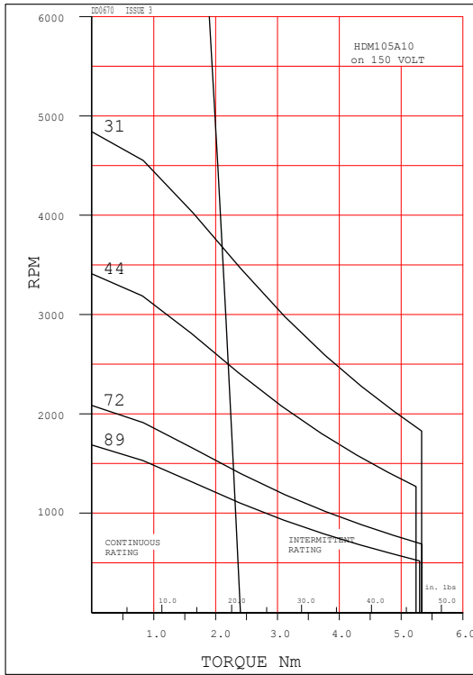
Performance Curve 150V
