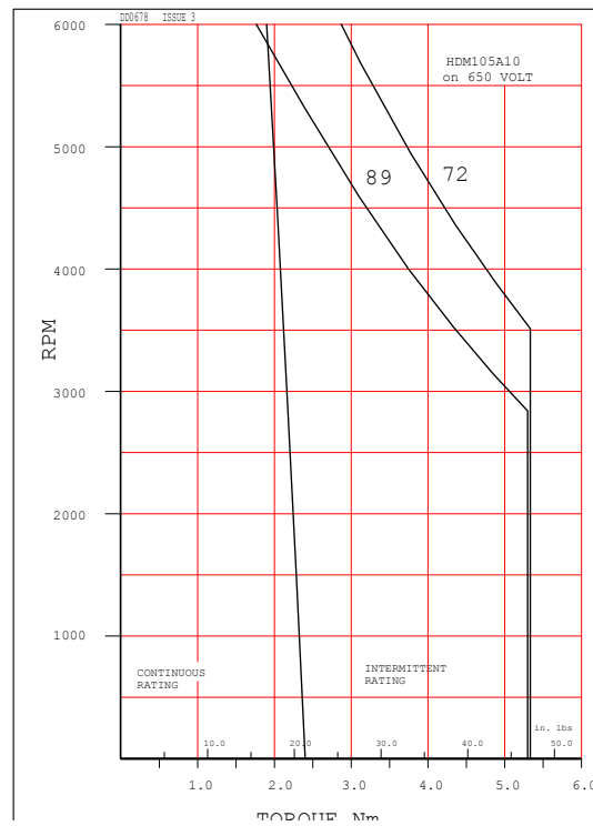
Performance Curve 650V
